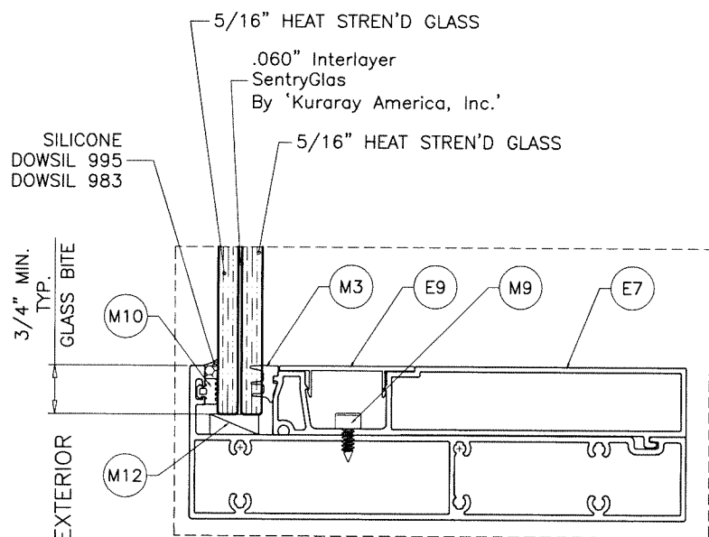
GLASS TYPE 'B' 11/16" OVERALL LAM. GLASS
