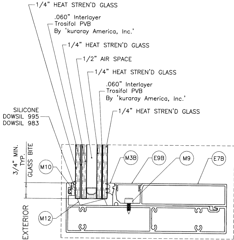
GLASS TYPE 'F' 1-1/2" OVERALL INSUL. LAM. GLASS
