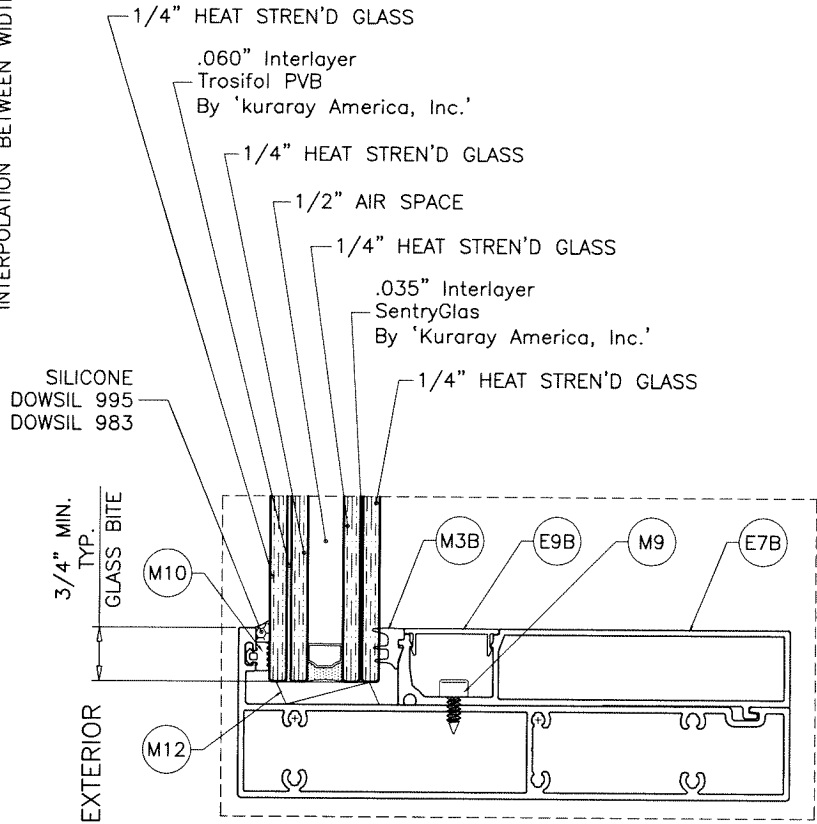
GLASS TYPE 'E' 1-1/2" OVERALL INSUL. LAM. GLASS
