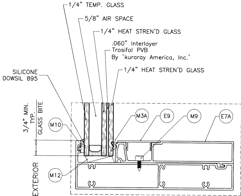
GLASS TYPE 'D1' 1-7/16" OVERALL INSUL. LAM. GLASS
