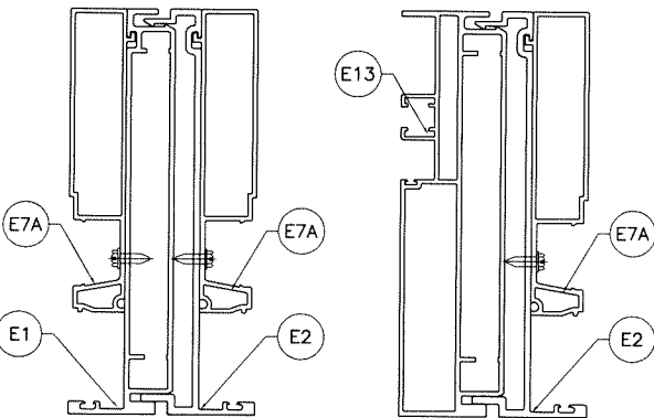
MULLION 'M1C'
