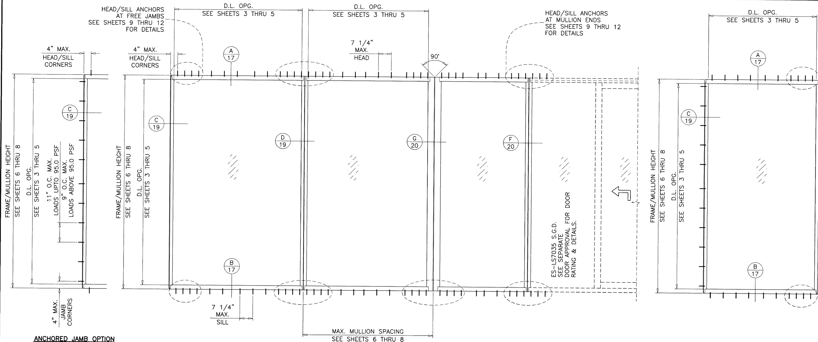
TYPICAL ELEVATIONS WITHOUT RECEPTORS
